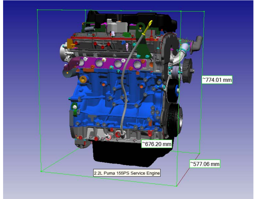
2.2-litre Ford Duratorq TDCi 155ps (Euro Stage 5)
